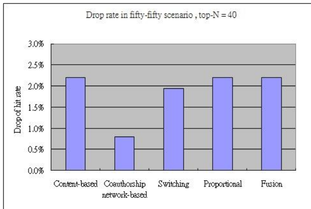
Figure 6. Drop of hit rate in fifty-fifty scenario
