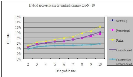
Figure 5. The result of various methods in diversified scenario when top-N = 10
