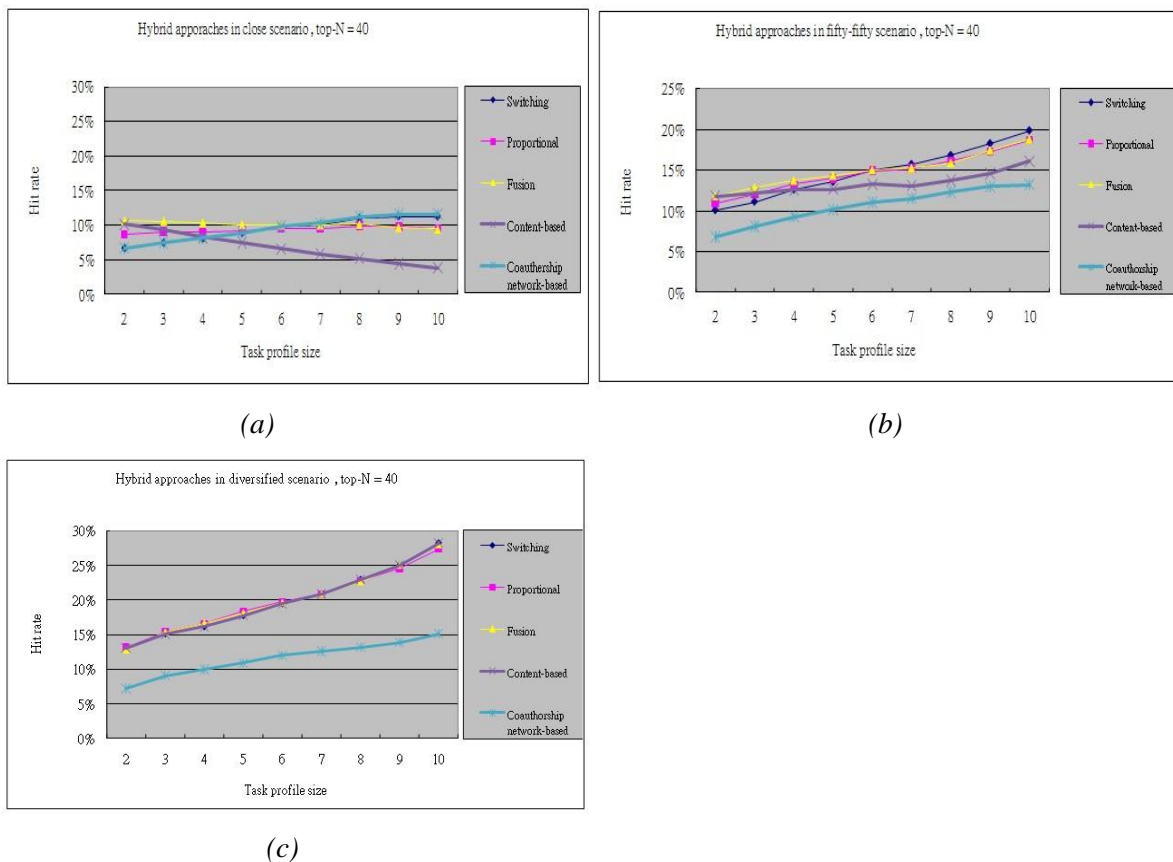
Figure 4. Hit rates of the three hybrid methods for recommending top-40 articles using content-based and coauthorship network-based approaches as benchmark under (a) close scenario (b) fifty-fifty scenario (c) diversified scenario
