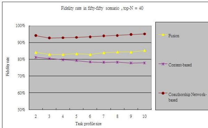
Figure 8. The fidelity rate of fusion in fifty-fifty scenario
