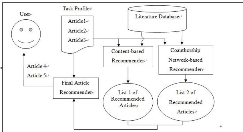
Figure 1. Architecture of the proposed recommendation framework
